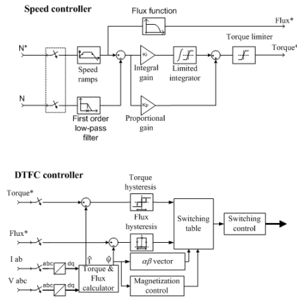
Controller schematics
